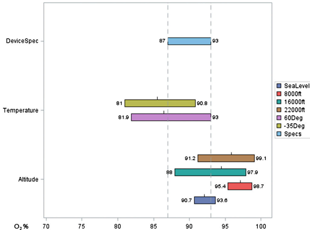
FIGURE 3. Range and mean FIO 2 on the 192 mL bolus setting with the Eclipse at a respiratory rate of 30 during all test conditions.
