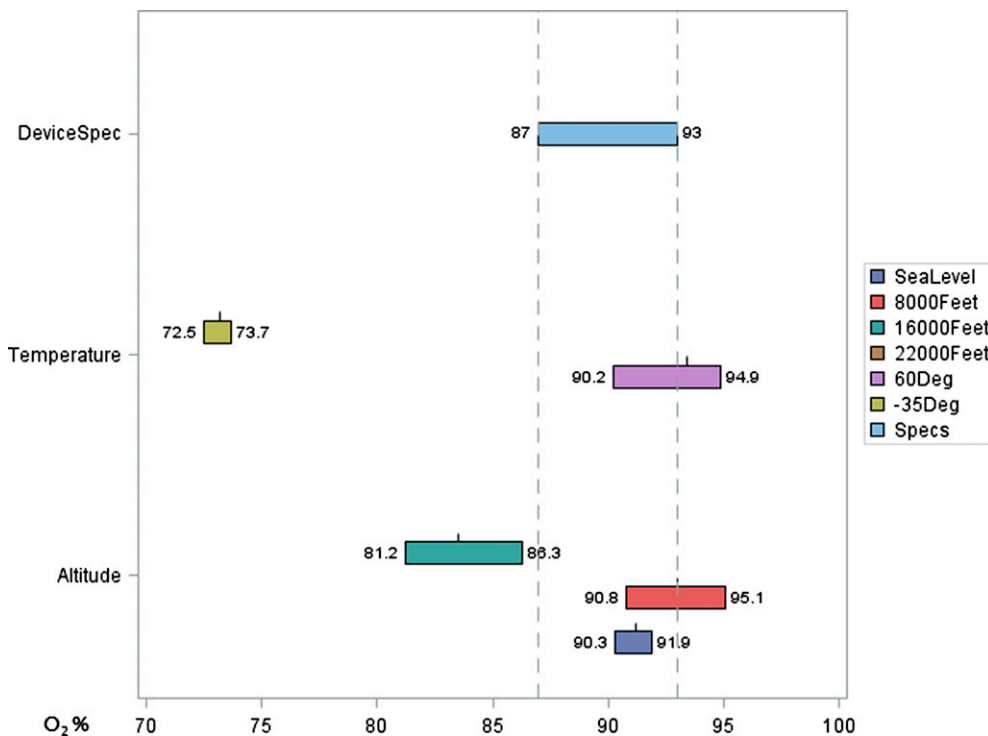
FIGURE 5. Range and mean FIO 2 at the 3 L/min continuous flow setting with the iGo at a respiratory rate of 30 during all test conditions.
