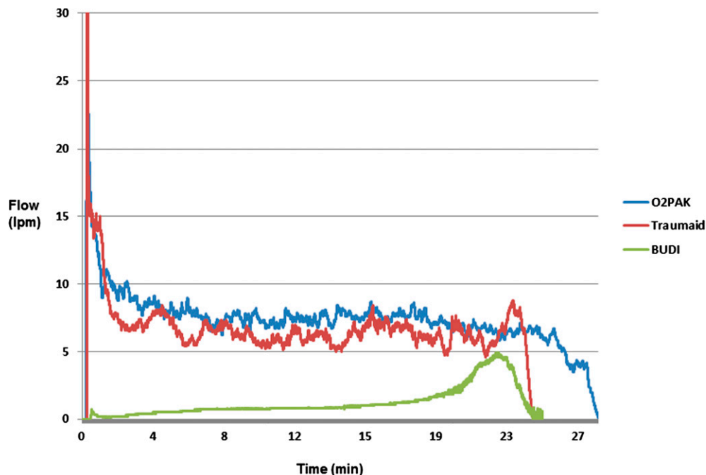
FIGURE 6. Sample run with all 3 chemical oxygen generators showing flow rates and duration of operation.
