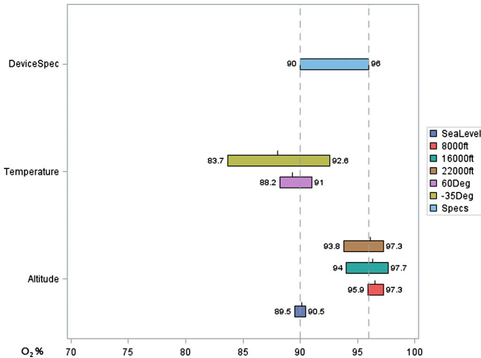
FIGURE 4. Range and mean FIO 2 on the 96 mL bolus setting with the Sacros at a respiratory rate of 30 during all test conditions.
